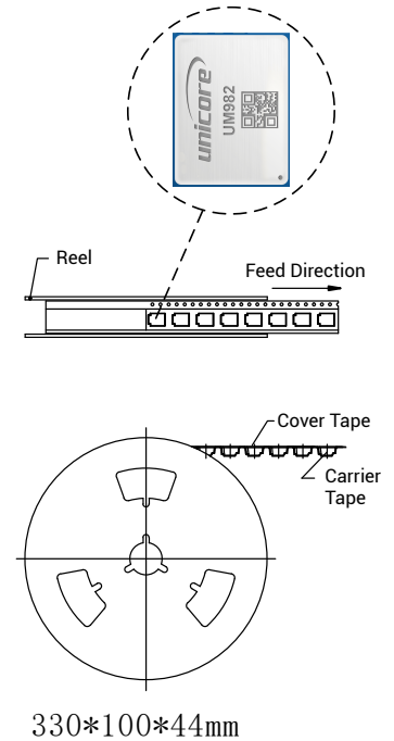
Reel Packaging Diagram (For Reference Only)
