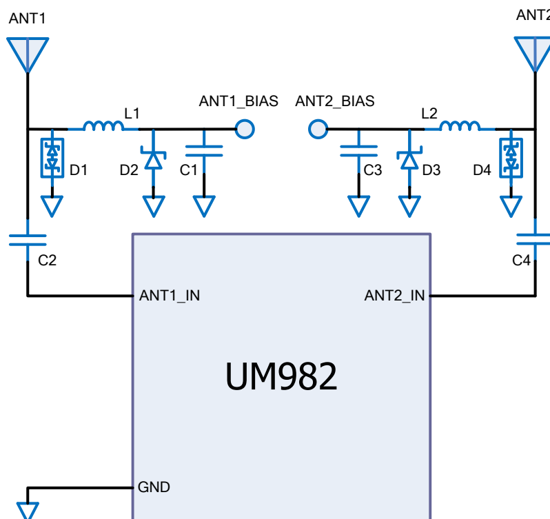
Figure 3-2 UM982 External Antenna Feed Reference Circuit
