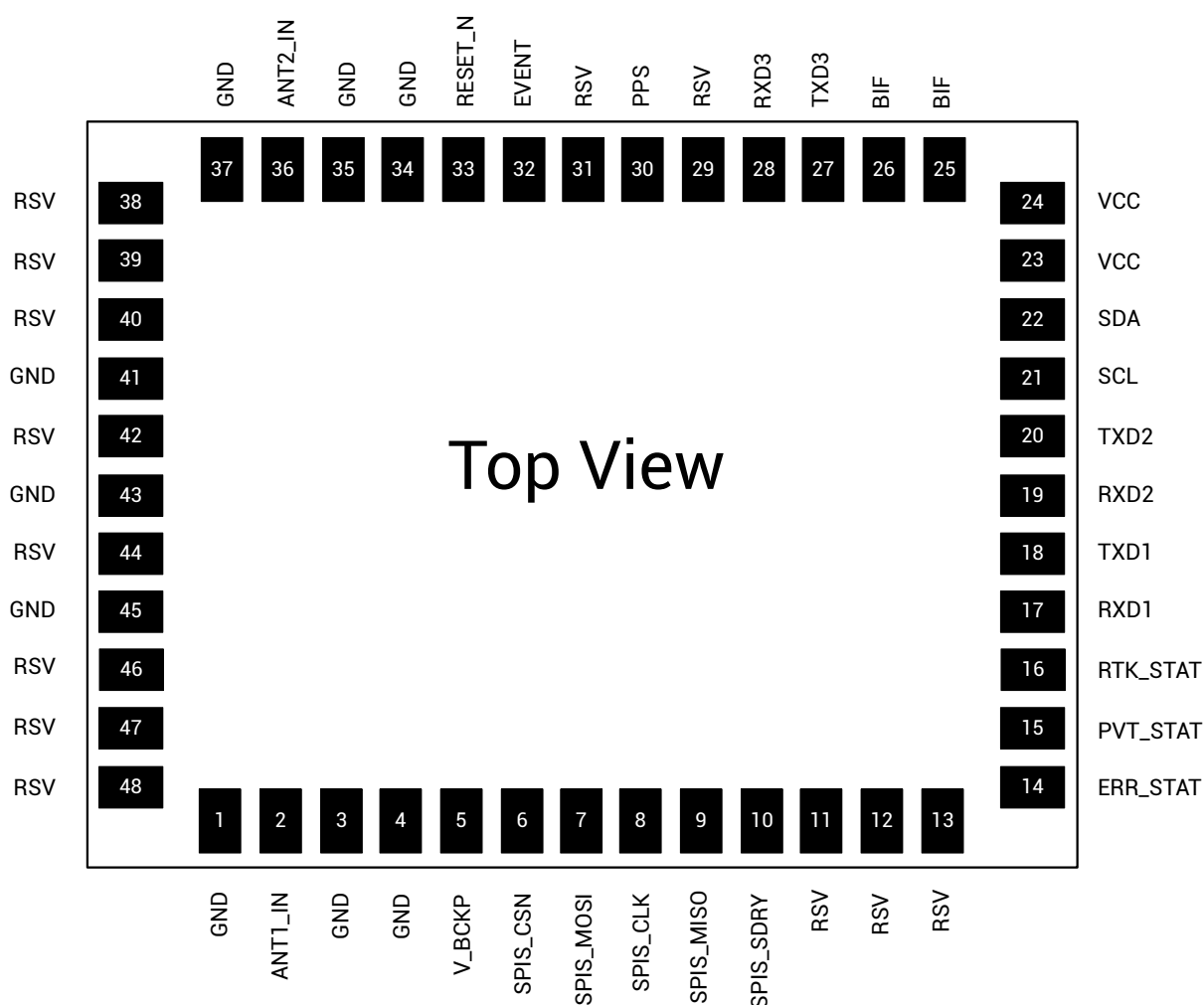
Figure 2-1 UM982 Pins
